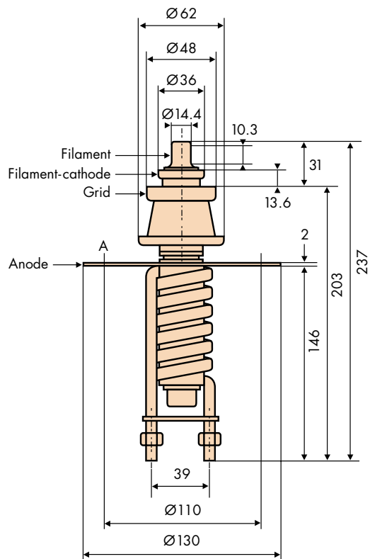
Outline drawing (mm)
